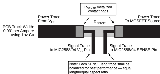
Figure 6. 4-Wire Kelvin Sense Connections for R_{\text{SENSE}} Protection Against Voltage Transients
