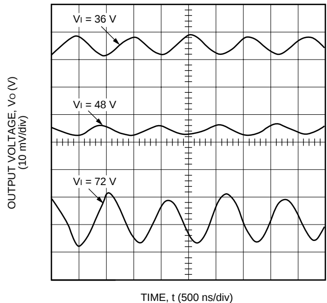
Figure 4. Typical FW250R1 Output Ripple Voltage at Room Temperature, and Full Load Output
