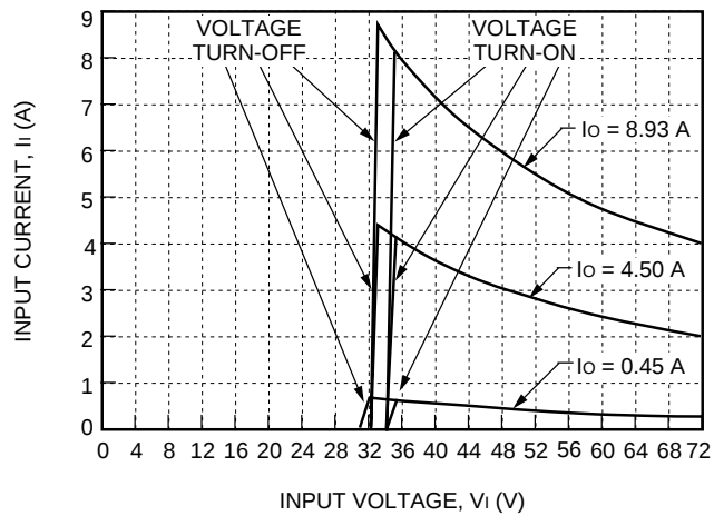
Figure 1. Typical FW250R1 Input Characteristics at Room Temperature
