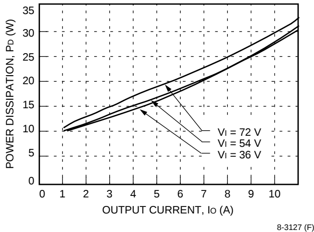
Figure 24. FW300R1 Power Dissipation vs. Output Current at 25 °C
