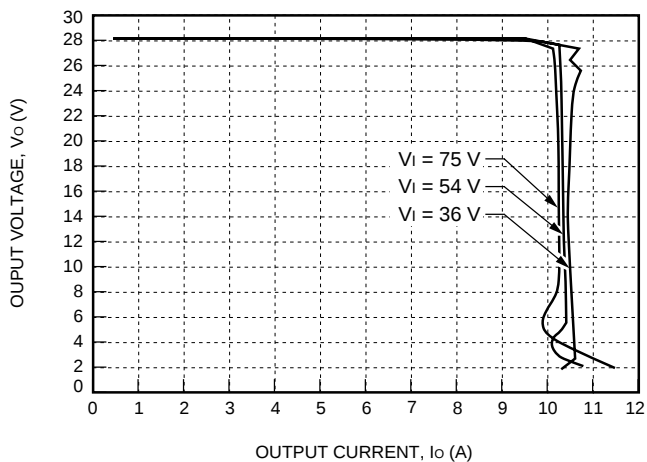
Figure 2. Typical FW250R1 Output Characteristics at Room Temperature
