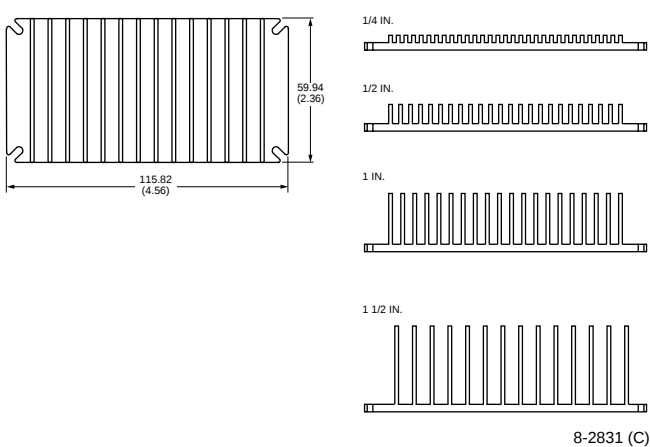
Figure 27. Transverse Heat Sink
