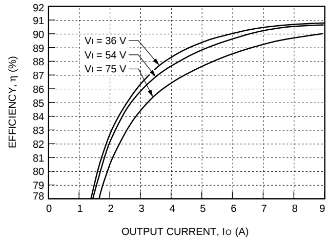
Figure 3. Typical FW250R1 Efficiency vs. Output Current at Room Temperature
