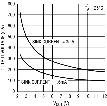
RESET, FAULT, COMPOUT Output Voltage vs V_{CC1}
