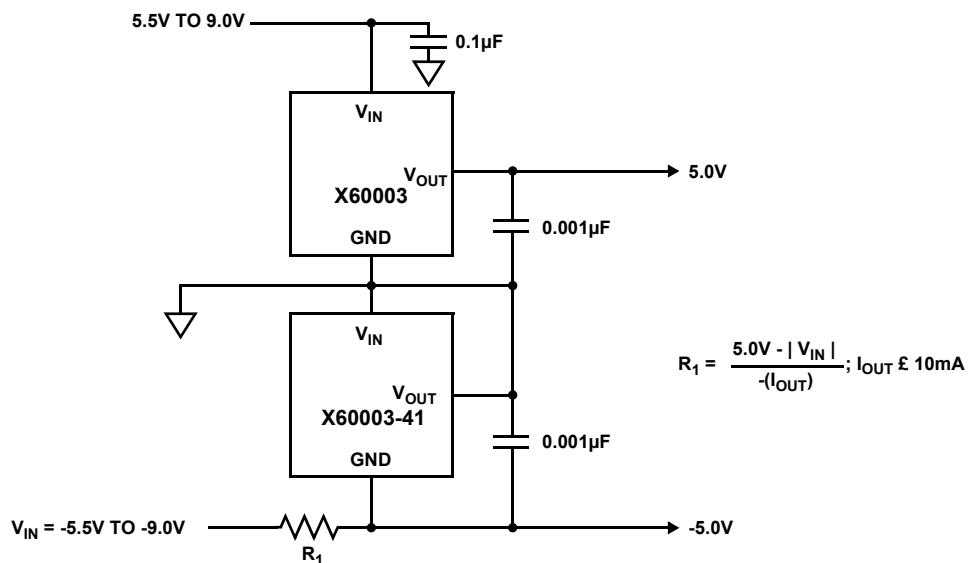
FIGURE 37. \pm 5.0V DUAL OUTPUT, HIGH ACCURACY REFERENCE
