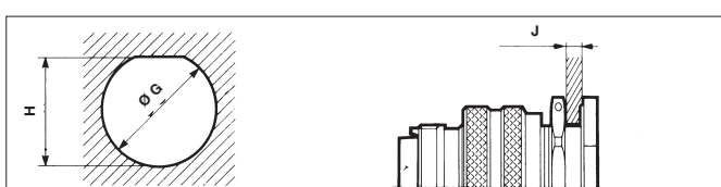
panel cut-out
