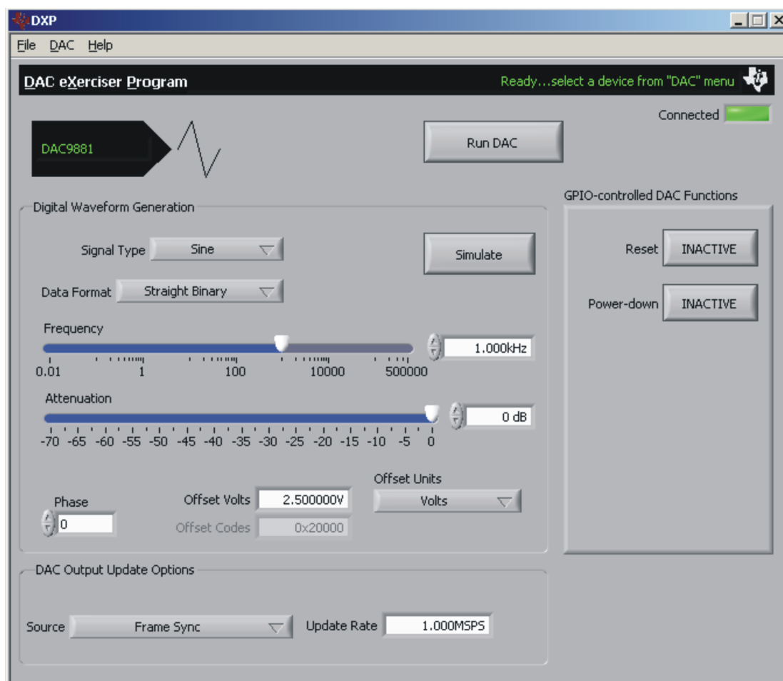
Figure 3. DAC8x11 EVM – Frequency/Amplitude and Update Rate Adjustments
