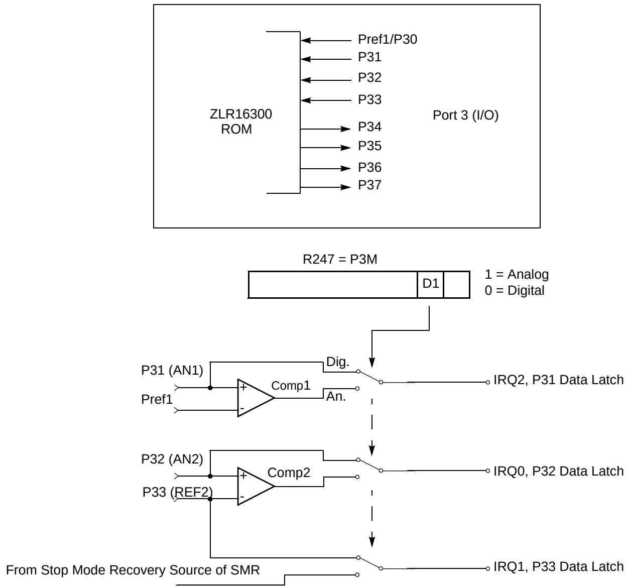
Figure 7. Port 3 Configuration
