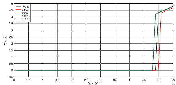
Figure 10-3. V_{CC} vs V_{SUP} Across Temperature
