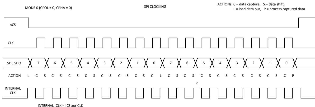
Figure 9-10. SPI Clocking
