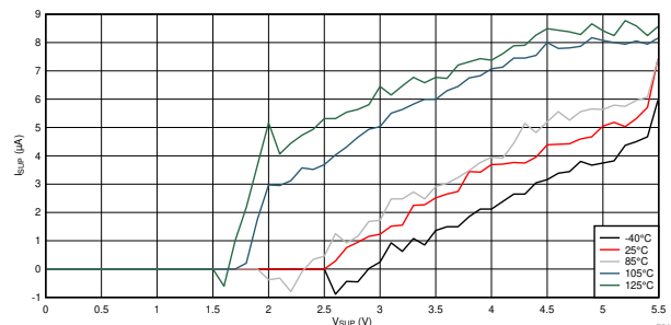
Figure 10-7. I_{SUP} vs V_{SUP} Across Temperature
