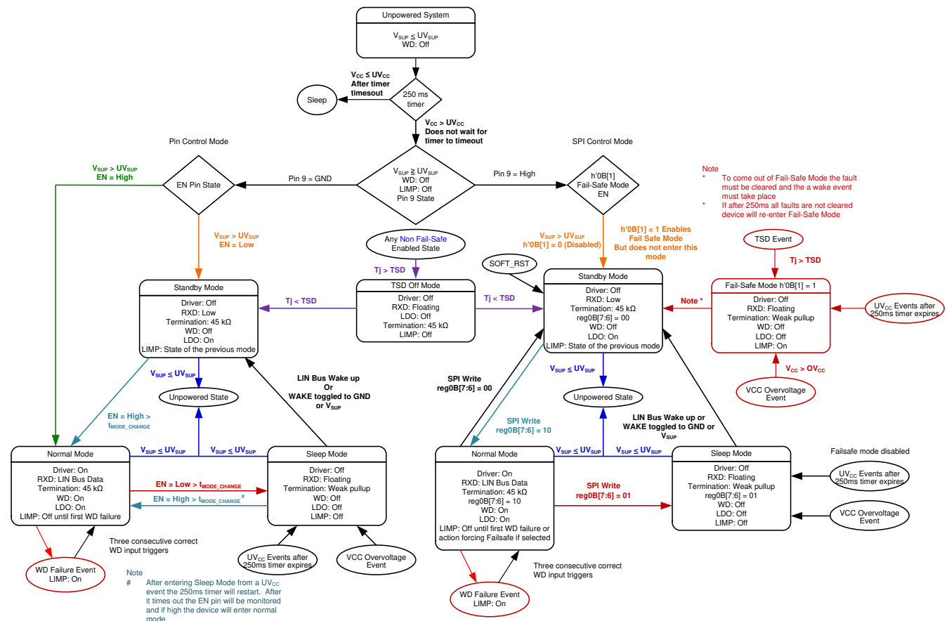
Figure 9-7. State Diagram with Failsafe
