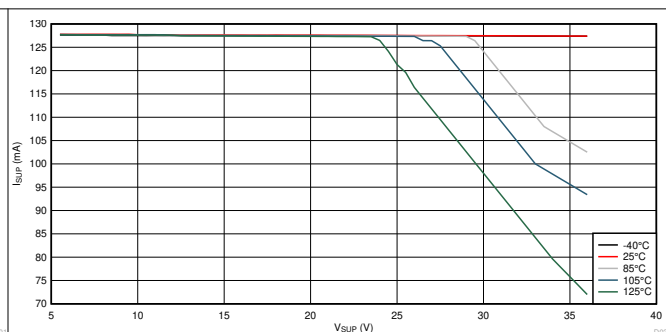
V_{CC} = 3.3\text{ V} I_{CC}\text{ Load} = 125\text{ mA} Normal Mode Figure 7-2. I_{SUP} vs V_{SUP} Across Temperature
