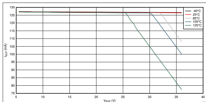
V_{CC} = 5\text{ V} I_{CC}\text{ Load} = 125\text{ mA} Normal Mode Figure 7-1. I_{SUP} vs V_{SUP} Across Temperature
