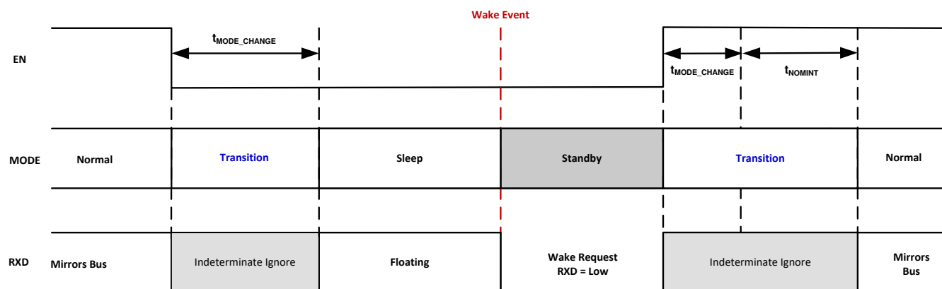
Figure 8-15. Mode Transitions
