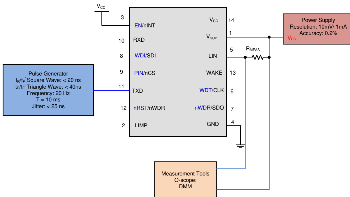
Figure 8-6. Test Circuit for I_{BUS\_LIM} at Dominant State (Driver on)
