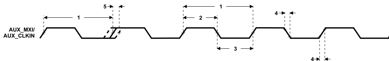
Figure 7-17. AUX_MXI/AUX_CLKIN Timing
