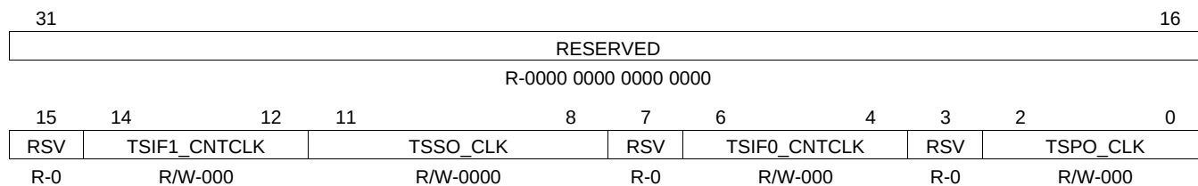
Figure 4-3. TSIFCTL Register [0x01C4 0050]
