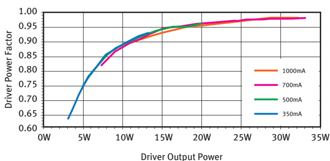
Driver Power Factor Characteristic at 230V Input
