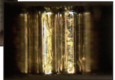
Gross Deformation of Crimped Terminal Resulting from Material Buildup in Crimper
