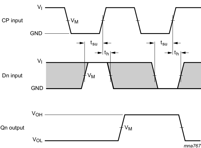
Measurement points are given in Table 8 . The shaded areas indicate when the input is permitted to change for predictable output performance. V_{OL} and V_{OH} are typical voltage output levels that occur with the output load.
