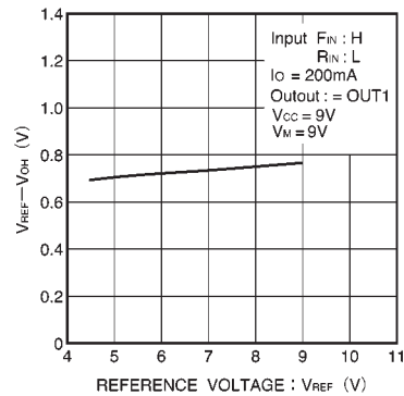
Fig.8 V_{REF} - V_{OH} voltage vs. V_{REF} reference voltage
