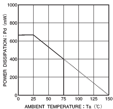
Fig.3 Thermal derating
