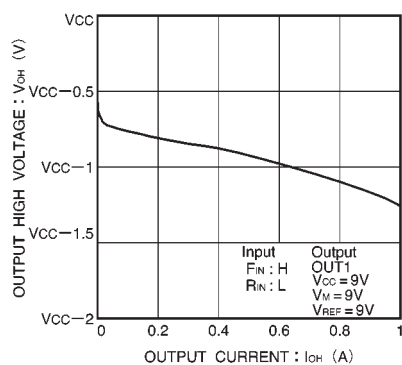
Fig.5 Output high level voltage vs. output current
