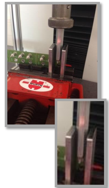
Shearforce
