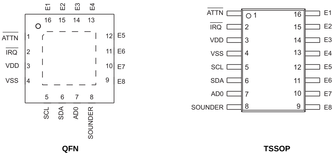
Figure 3. Package Pinouts
