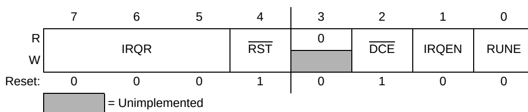
Figure 19. Configuration Register
