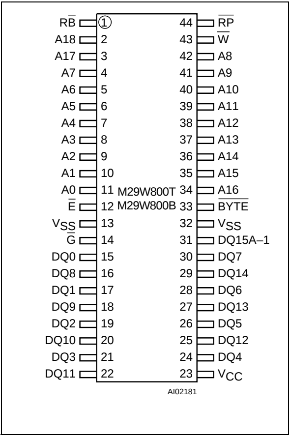
Figure 4. SO Connections
