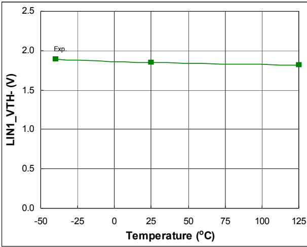
Fig. 53. Input Negative Going Threshold vs. Temperature
