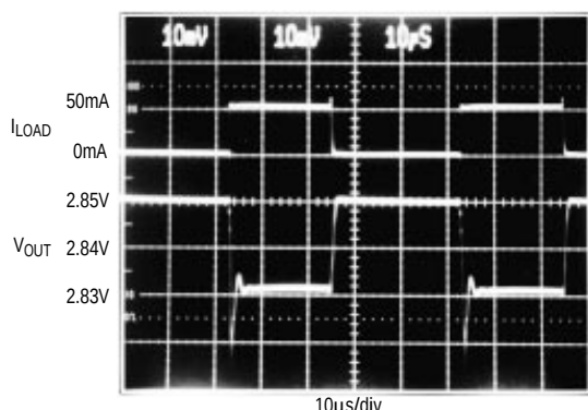
LOAD-TRANSIENT RESPONSE
