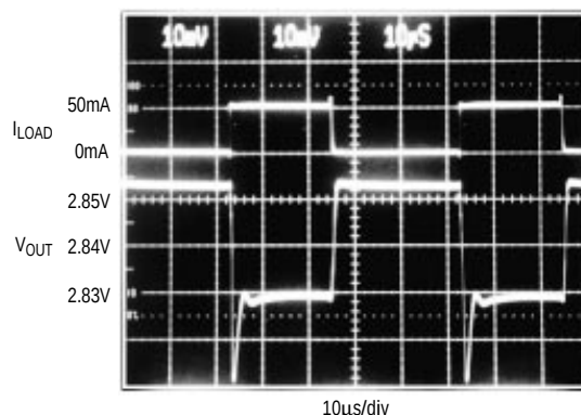
LOAD-TRANSIENT RESPONSE
