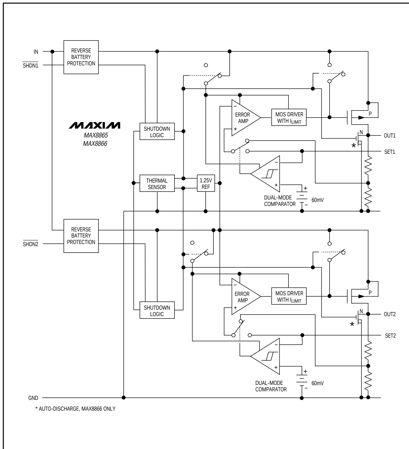
Figure 1. Functional Diagram
