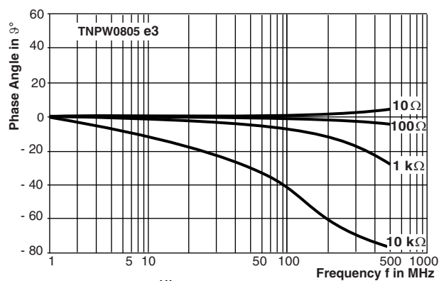
HF Performance (1)
