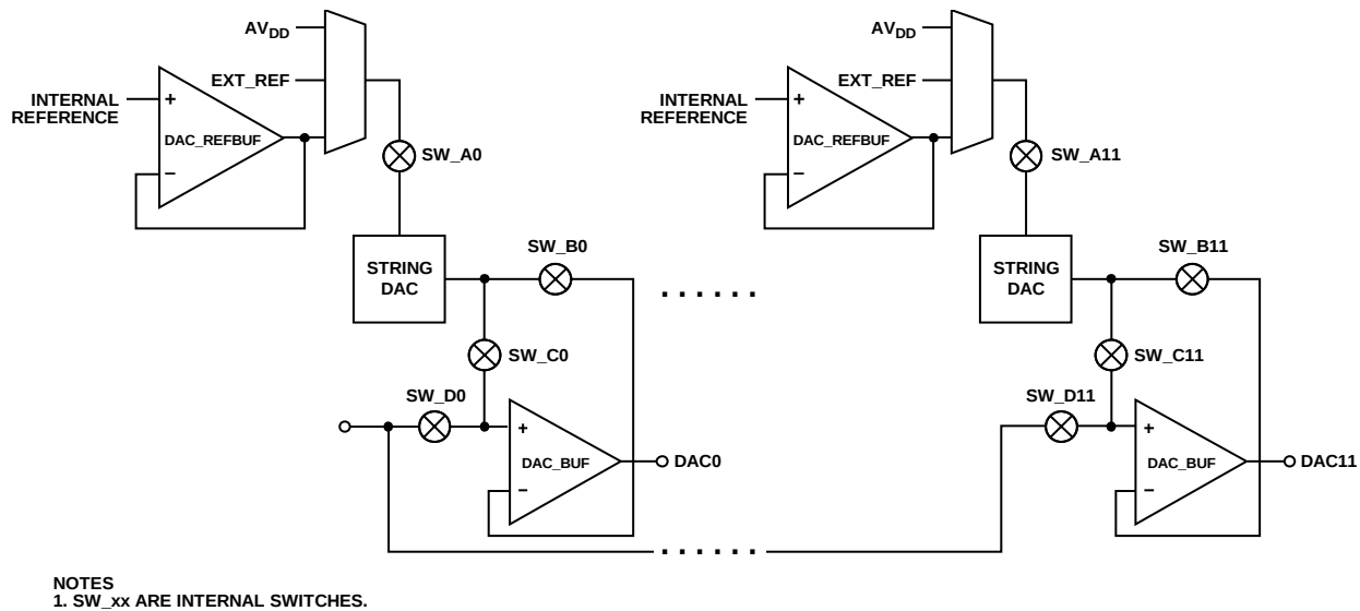
Figure 29. DAC Configuration
