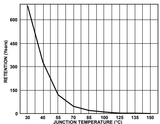
Figure 27. Flash/EE Memory Data Retention
