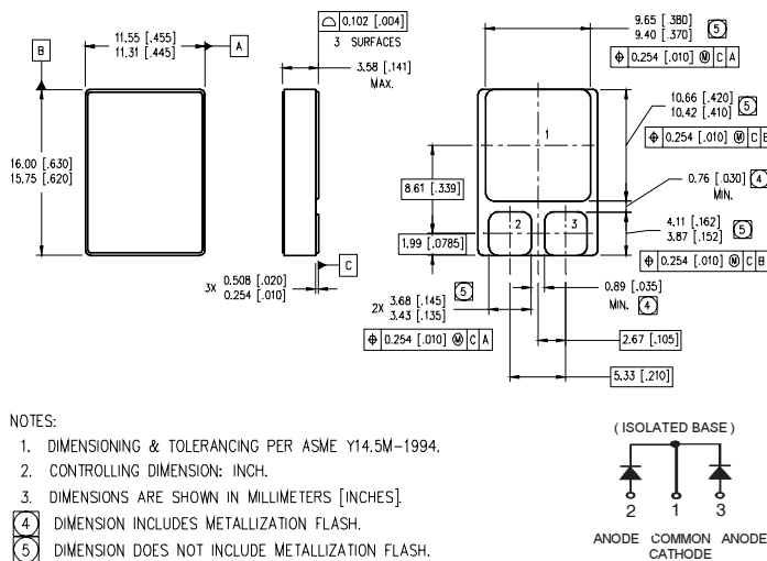
Case Outline and Dimensions - SMD-1
