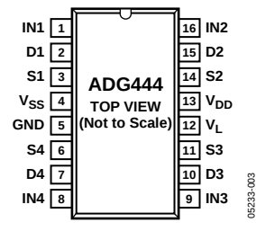
Figure 3. ADG444 (DIP/SOIC)
