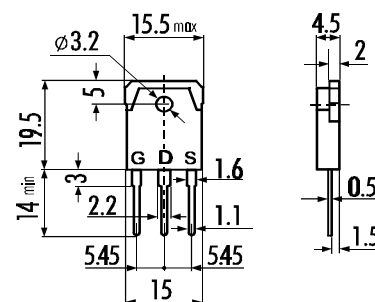
TO-3P
