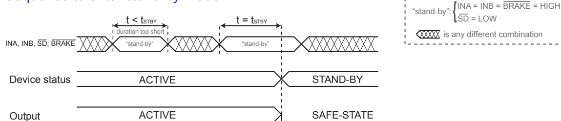
Figure 4. Standby state sequences
