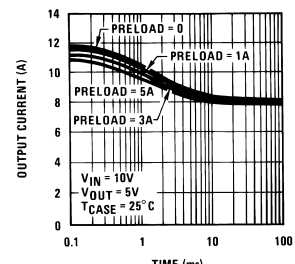
Current Limit
