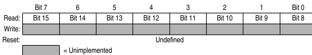
Figure 17-13. ATD Result Registers High
