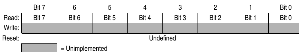
Figure 17-14. ATD Result Registers Low
