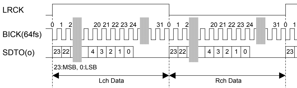
Figure 8. Mode 0 Timing
