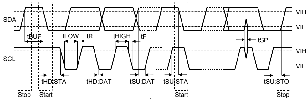
Figure 6. I²C Bus mode Timing
