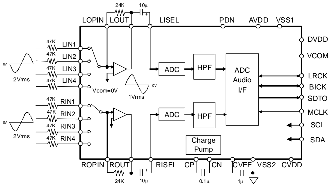
Figure 1. AK5367A Block Diagram
