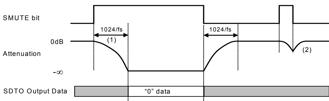
Figure 11. Soft Mute Function
