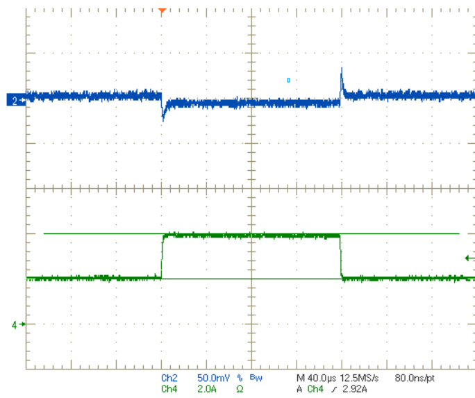
Figure 5. Step Response
