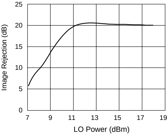
Image Rejection vs. LO Power F_{RF} = 30.3 \text{ GHz} , F_{LO} = 28 \text{ GHz} , P_{RF} = -10 \text{ dBm} Image Frequency = 25.7 \text{ GHz}
