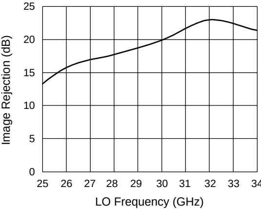
Image Rejection vs. LO Frequency F_{RF} = F_{LO} + 2 \text{ GHz} , P_{LO} = 12 \text{ dBm} Image Frequency = F_{LO} - 2 \text{ GHz}
