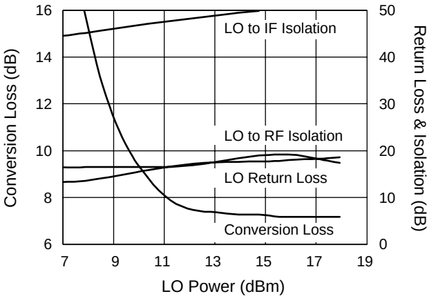
Performance vs. LO Power F_{RF} = 30.3 \text{ GHz} , F_{LO} = 28 \text{ GHz} , P_{RF} = -10 \text{ dBm}
