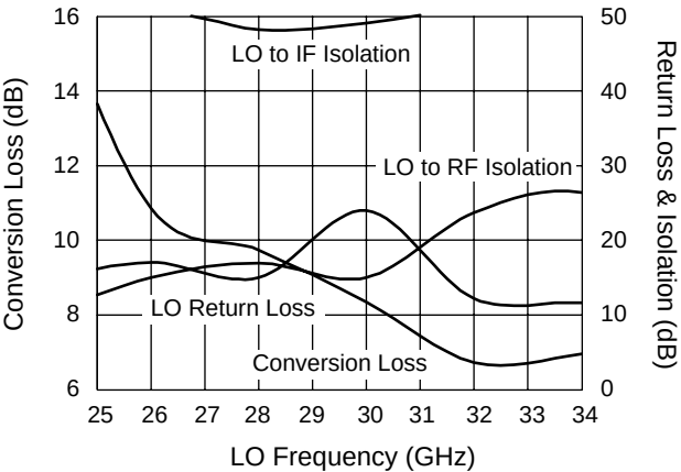
Performance vs. LO Frequency F_{RF} = F_{LO} + 2 \text{ GHz} , P_{LO} = 12 \text{ dBm}
