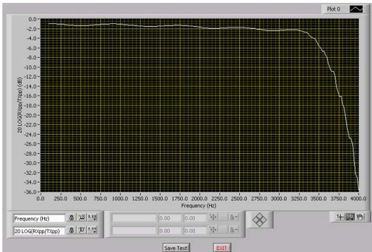
Figure 5. Transhybrid Loss
