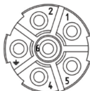
Female Insert
