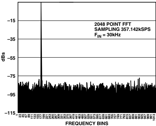
Figure 3. AD7810 SNR
