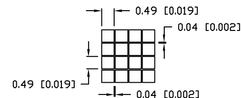
PIXEL DETAIL
