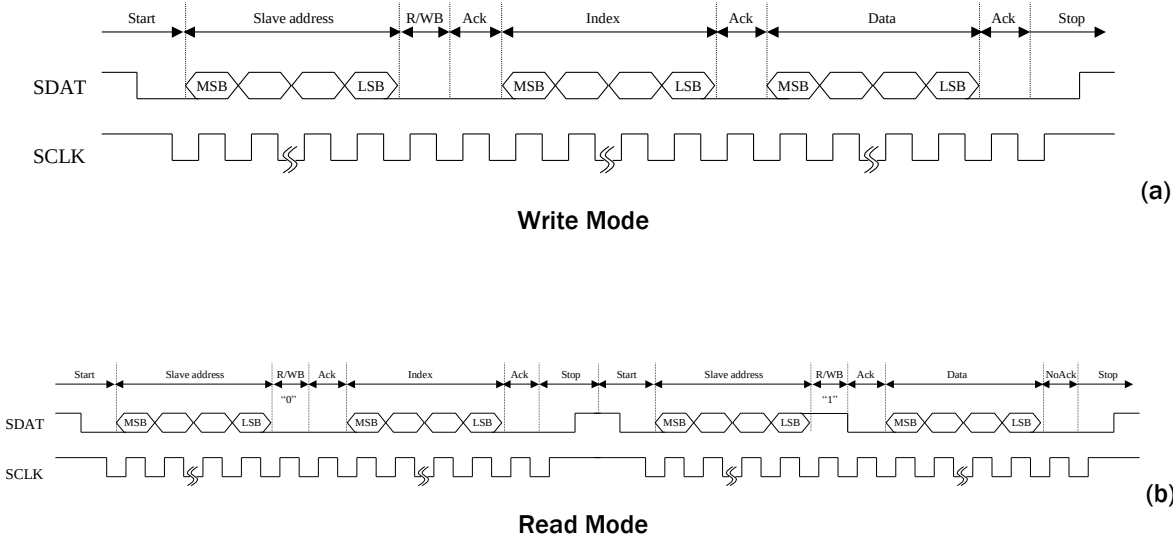
FIGURE 39. TIMING CHART OF SERIAL INTERFACE
