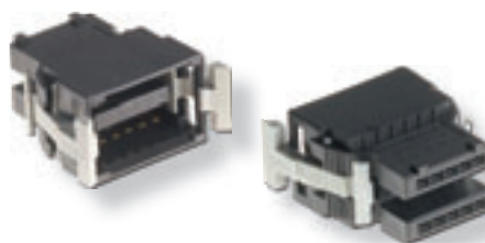
3 mm, 2 Sockets and 2 Plugs, 5 Position x 4
