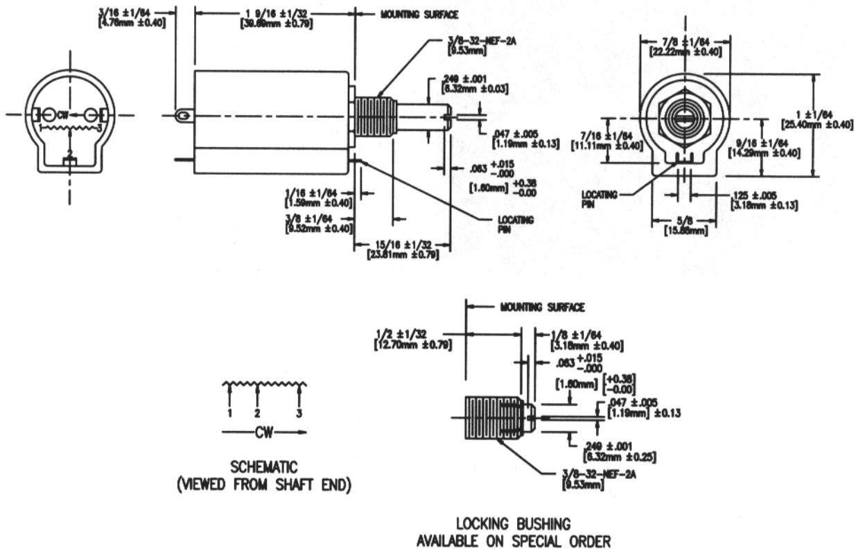
Figure 3 Series 62 Dimensions
