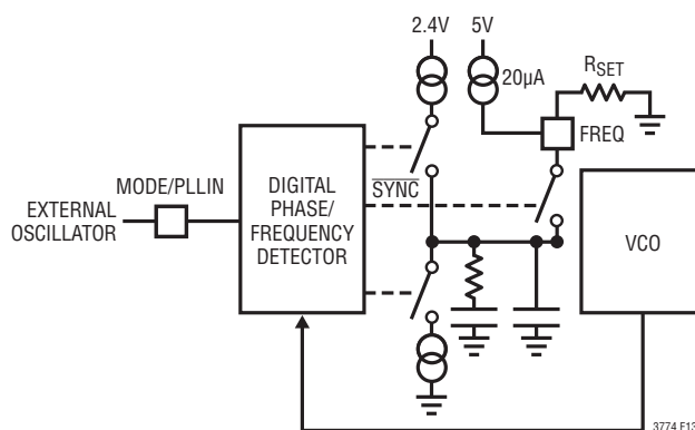
Figure 13. Phase-Locked Loop Block Diagram
