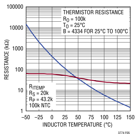
Figure 5. Resistance vs Temperature for the ITEMP Pin Network and the 100k NTC
