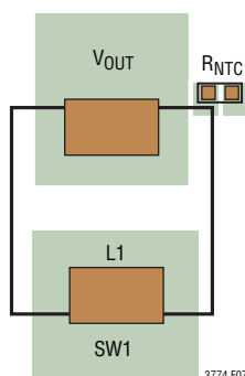
Figure 7. Thermistor Location. Place the Thermistor Next to the Inductor for Accurate Sensing of the Inductor Temperature, But Keep the ITEMP Pin Away from the Switch Nodes and Gate Drive Traces
