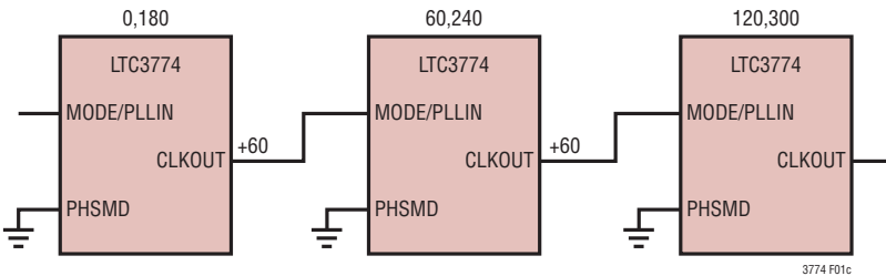
Figure 1c. 6-Phase Operation
