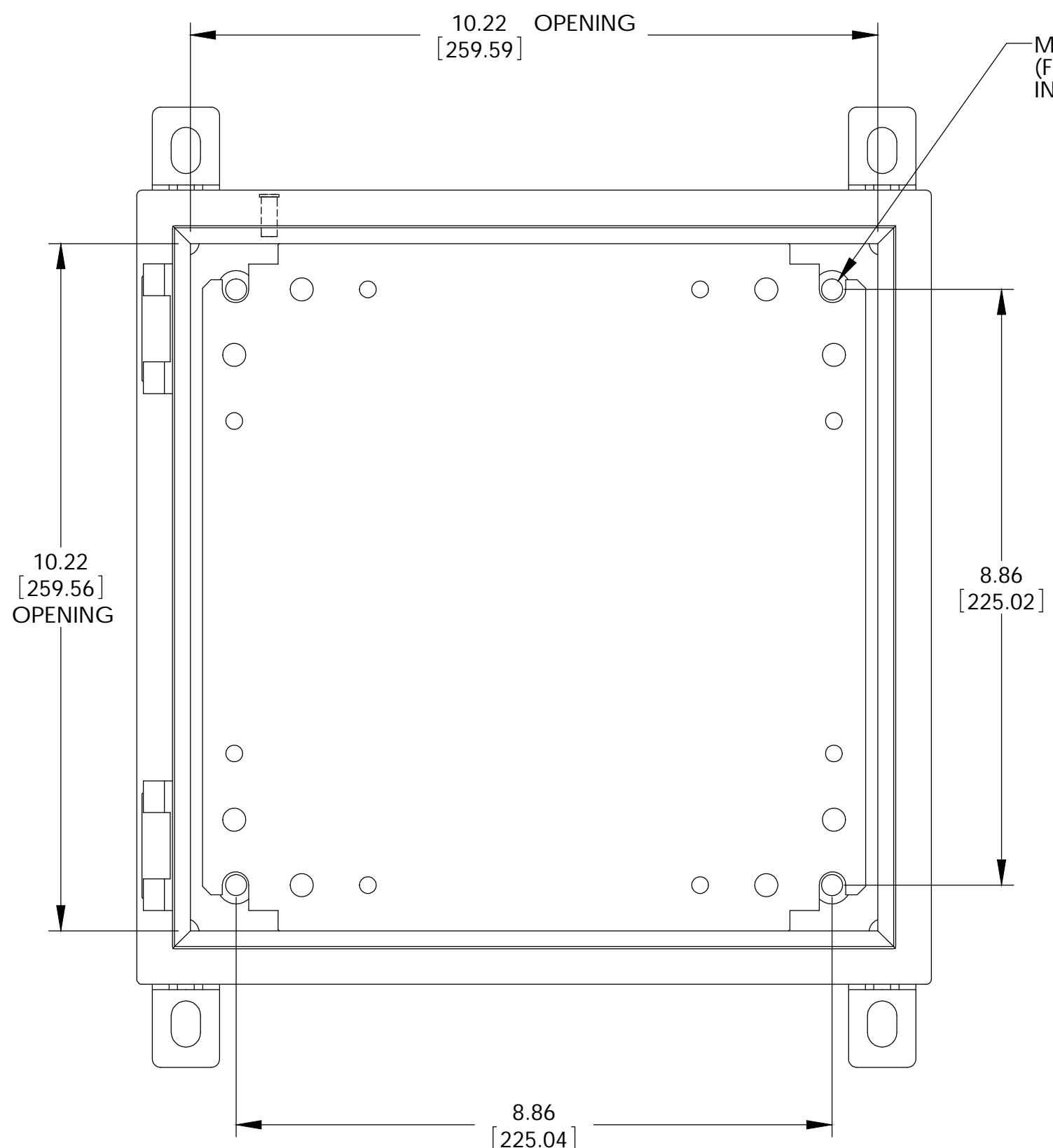
FRONT VIEW (LESS COVER)
