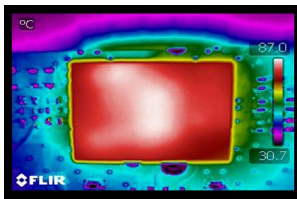
Figure 20 — Thermal Image ( V_{IN} = 24V , I_{OUT} = 4.2A , CR, OLFM Evaluation PCB)
