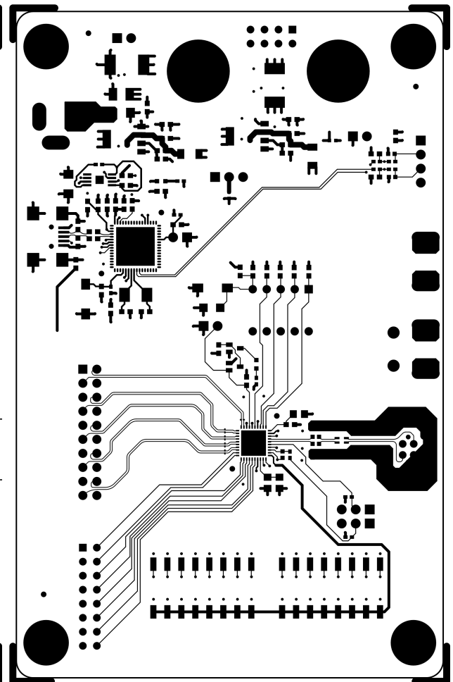
Figure C-2. Top Copper
