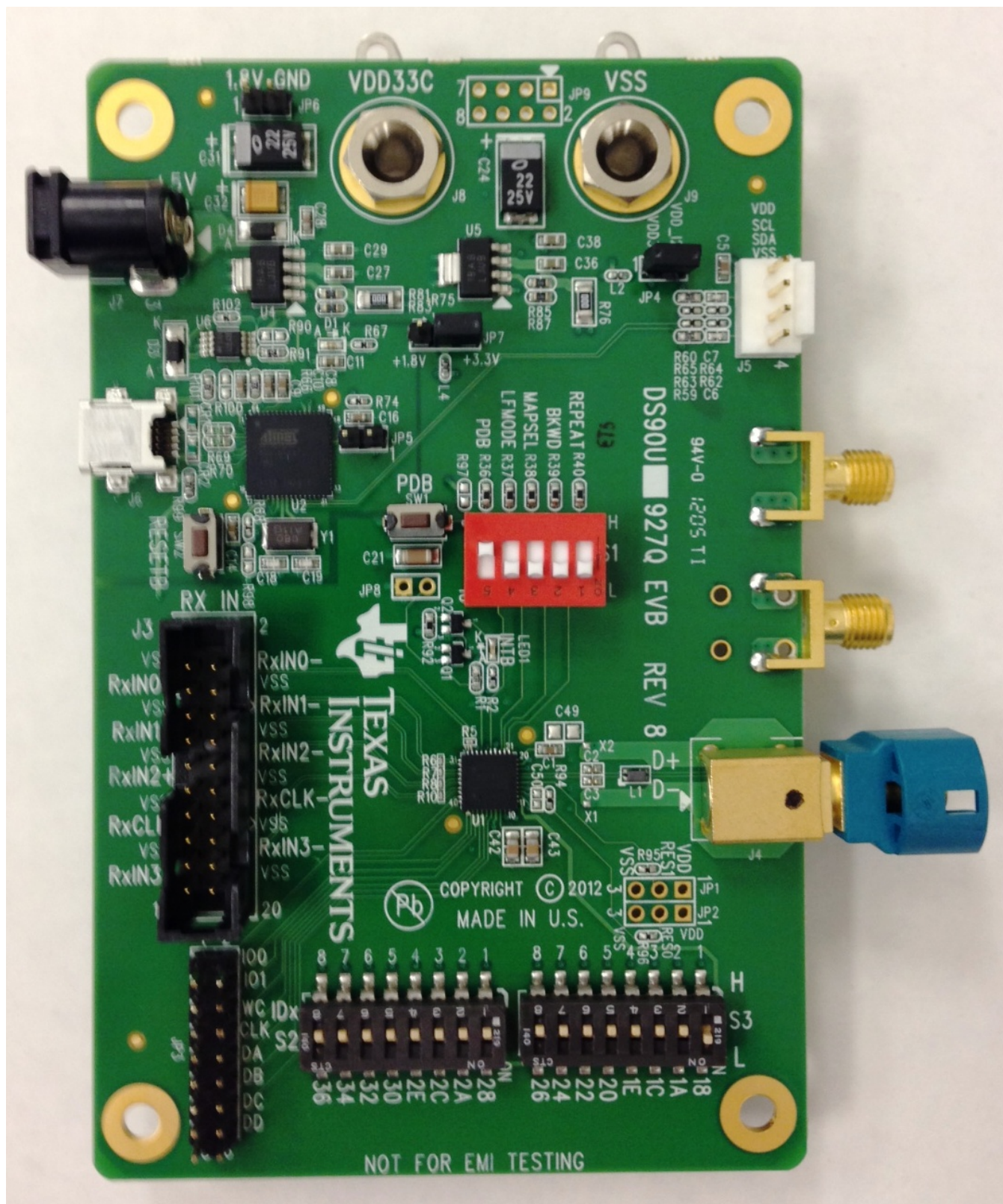
Figure 2-1. DS90UB927QEVMB
