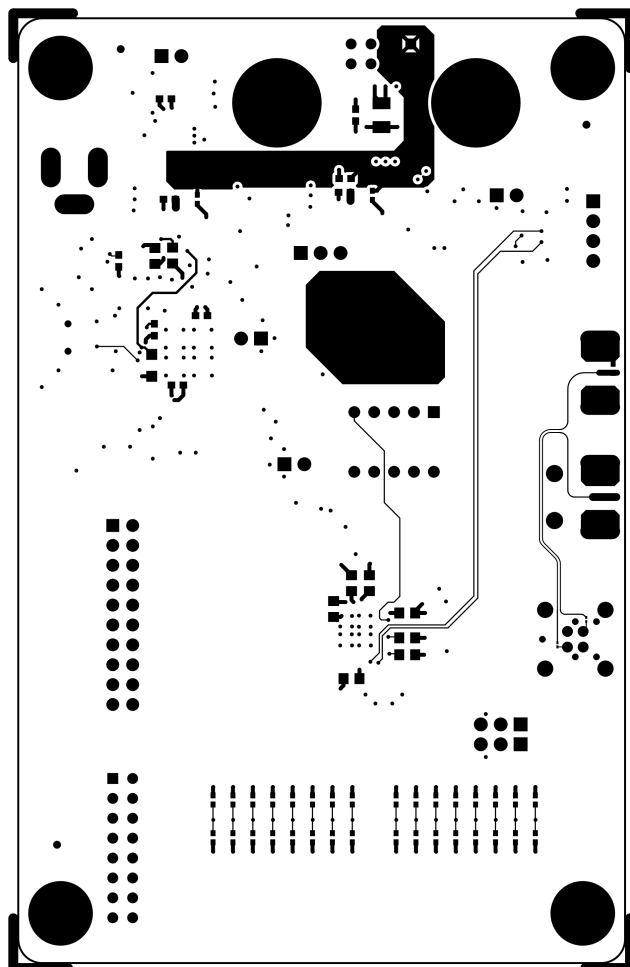
Figure C-5. Bottom Copper
