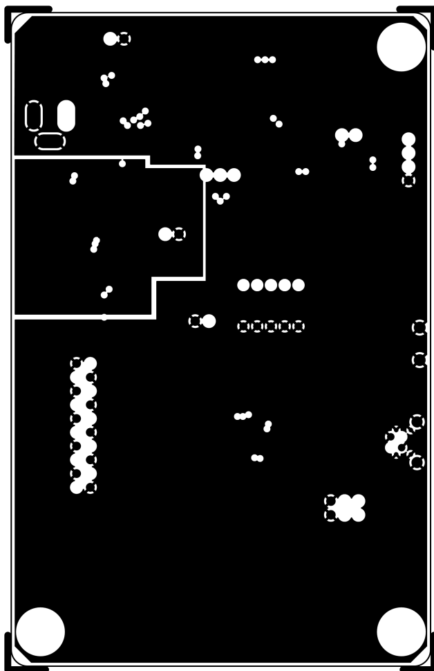
Figure C-3. Internal Layer 1: Ground
