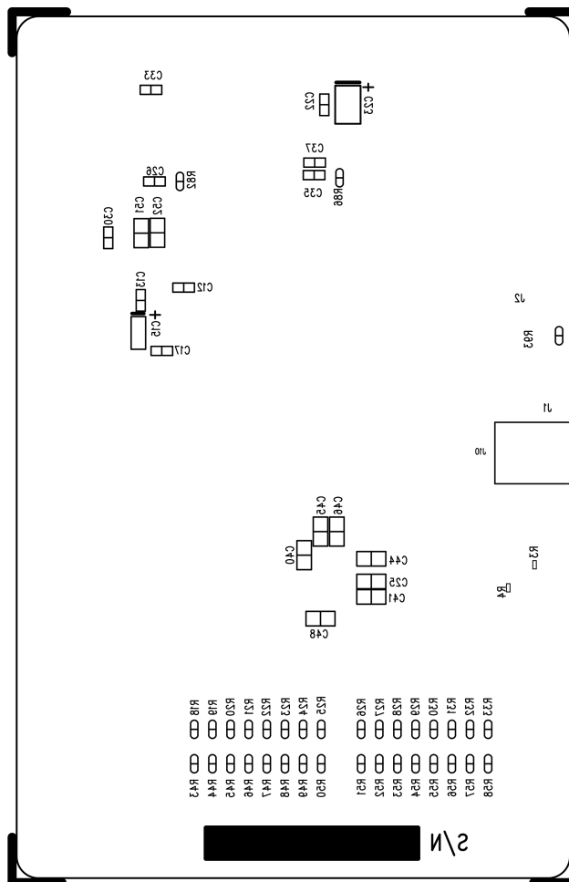
Figure C-6. Bottom Silkscreen
