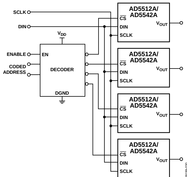
Figure 38. Addressing Multiple DACs
