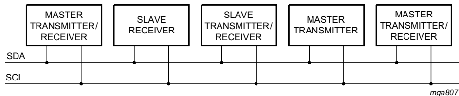
Fig 22. System configuration
