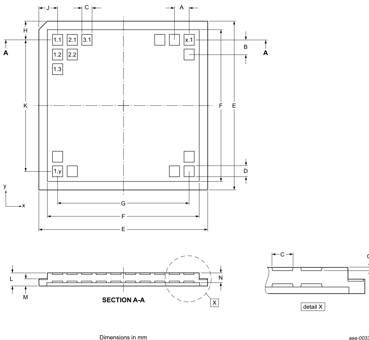
Fig 32. Tray details
