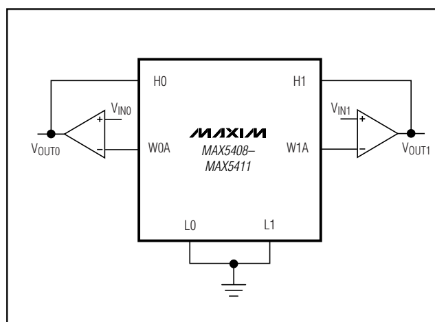
Figure 6. Gain Control
