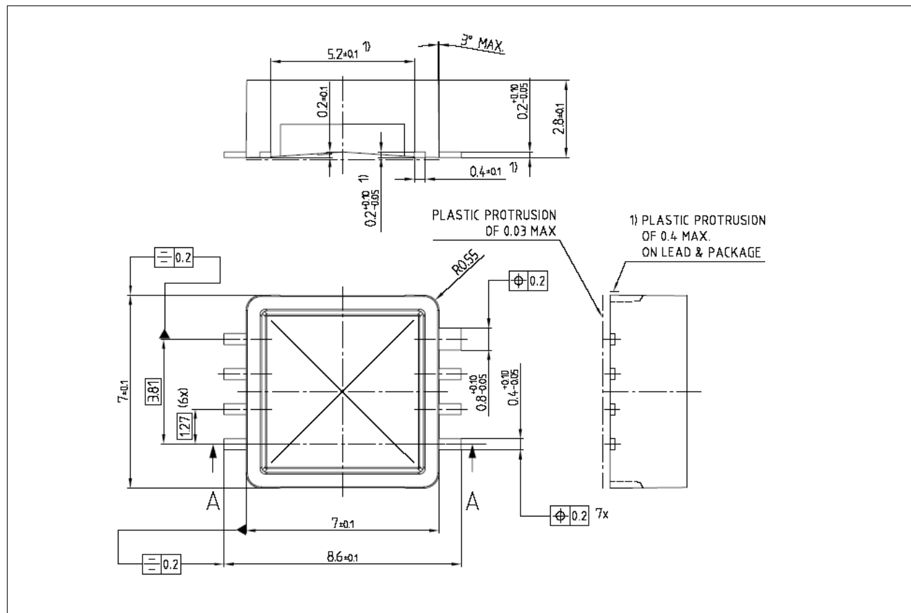
Figure 11 Package
