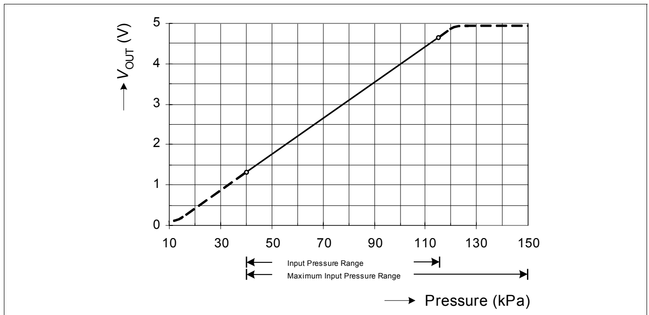
Figure 3 Transfer Function
