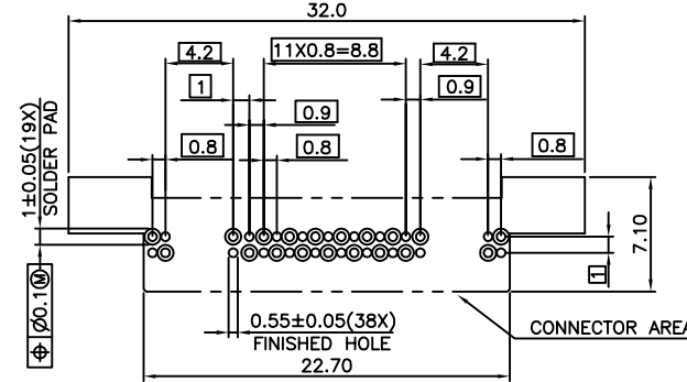
Required board layout View on backside
