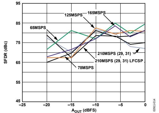
Figure 15. Dual-Tone IMD vs. A_{OUT} @ f_{OUT} = f_{CLOCK}/7
