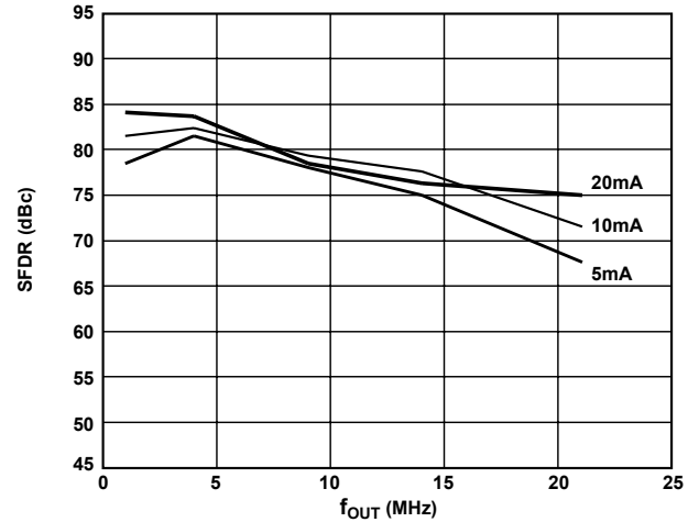
Figure 10. SFDR vs. f_{OUT} and I_{OUTS} @ 65 MSPS and 0 dBFS
