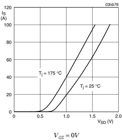
Fig 14. Reverse diode current as a function of reverse diode voltage; typical values
