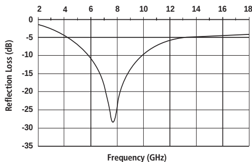
Q-Zorb Wave 0.060 in (1.5 mm) Thick P/N 2240
