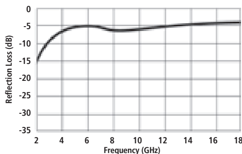
Q-Zorb .125 in (3.2 mm) Thick P/N 2242
