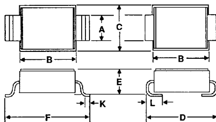
"C" BEND (MODIFIED J-BEND)
