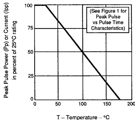
FIGURE 3 - Derating Curve
