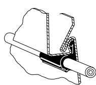
Horizontal Siding Clip
